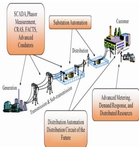
Figure 1. Components of smart grid.
